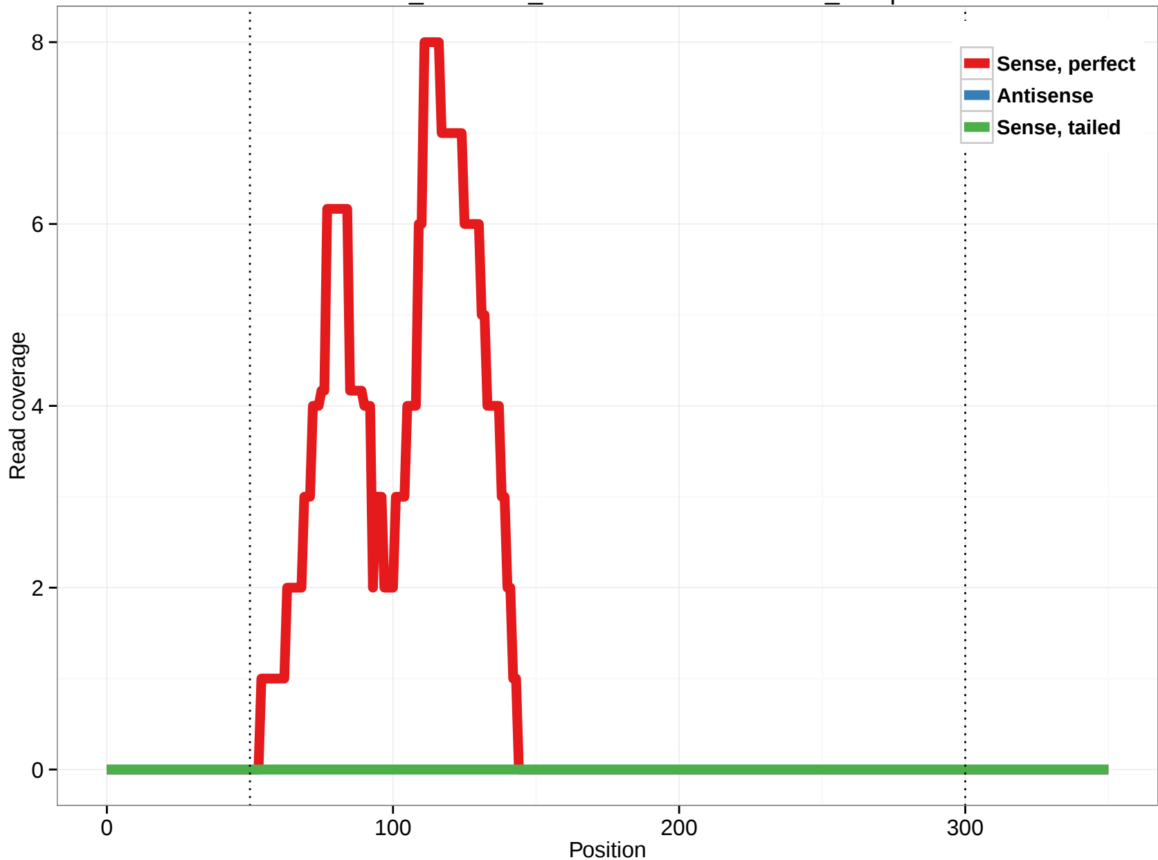
ornAna1_ensGene_ENSOANT00000002621_27.5p
