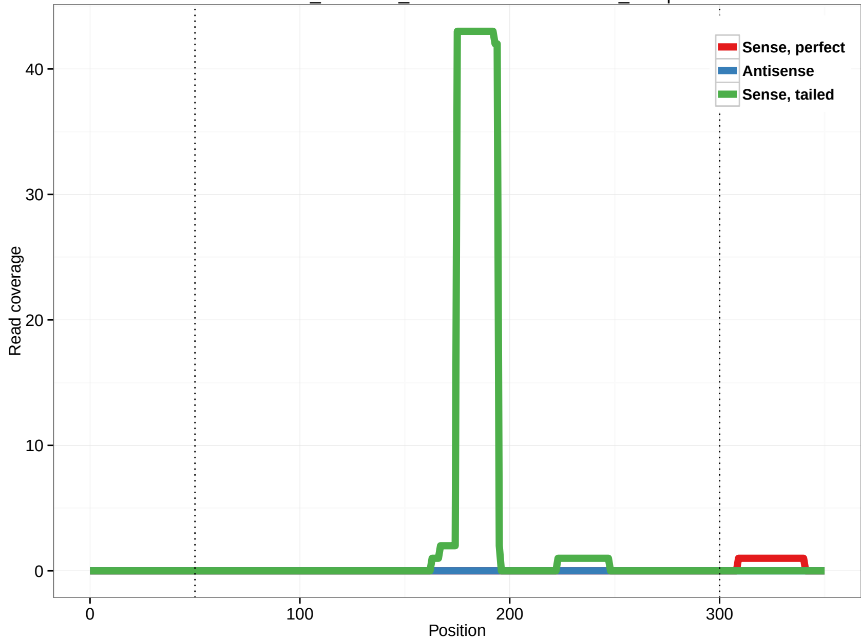
ornAna1_ensGene_ENSOANT00000002601_16.3p
