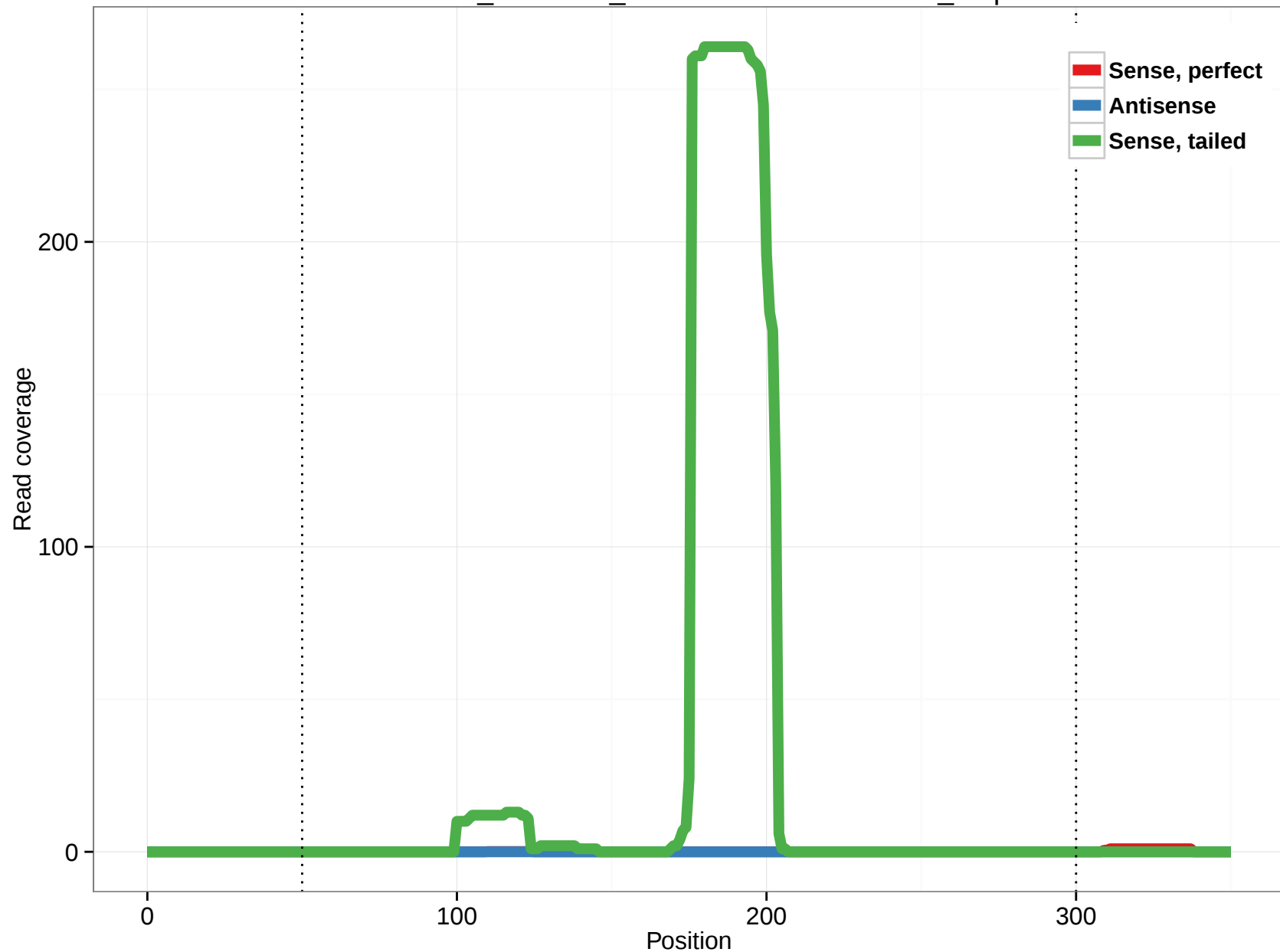
ornAna1_ensGene_ENSOANT00000002587_6.3p
