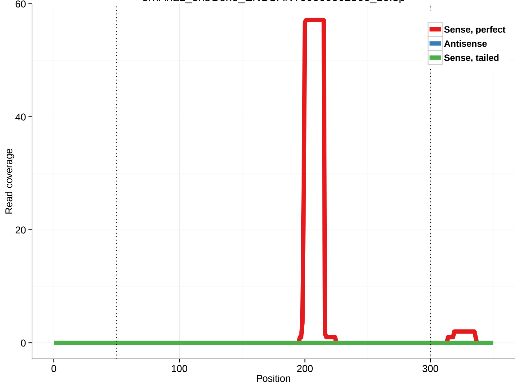
ornAna1_ensGene_ENSOANT00000002566_10.3p
