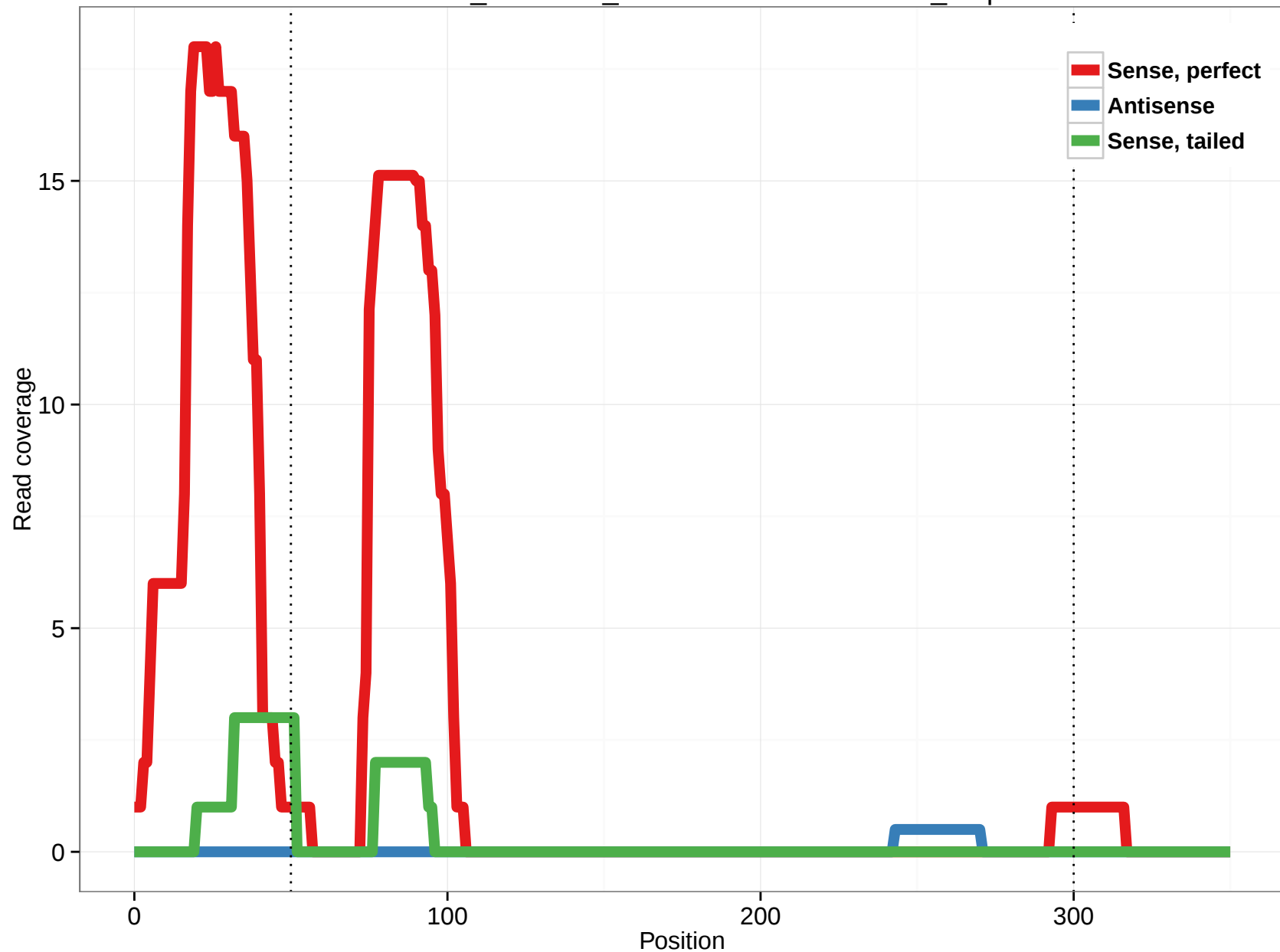
ornAna1_ensGene_ENSOANT00000002548_3.5p
