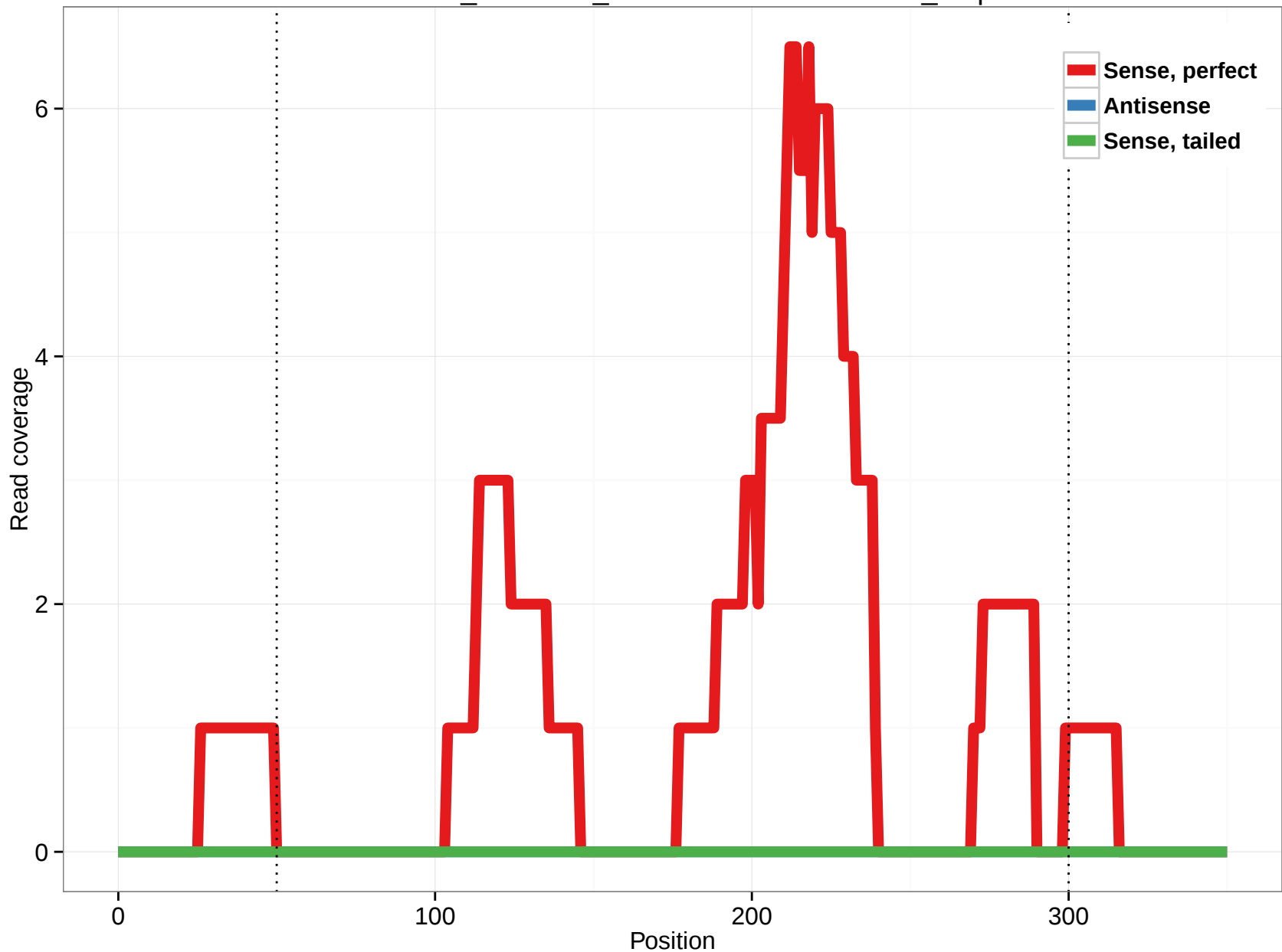
ornAna1_ensGene_ENSOANT00000002548_0.5p
