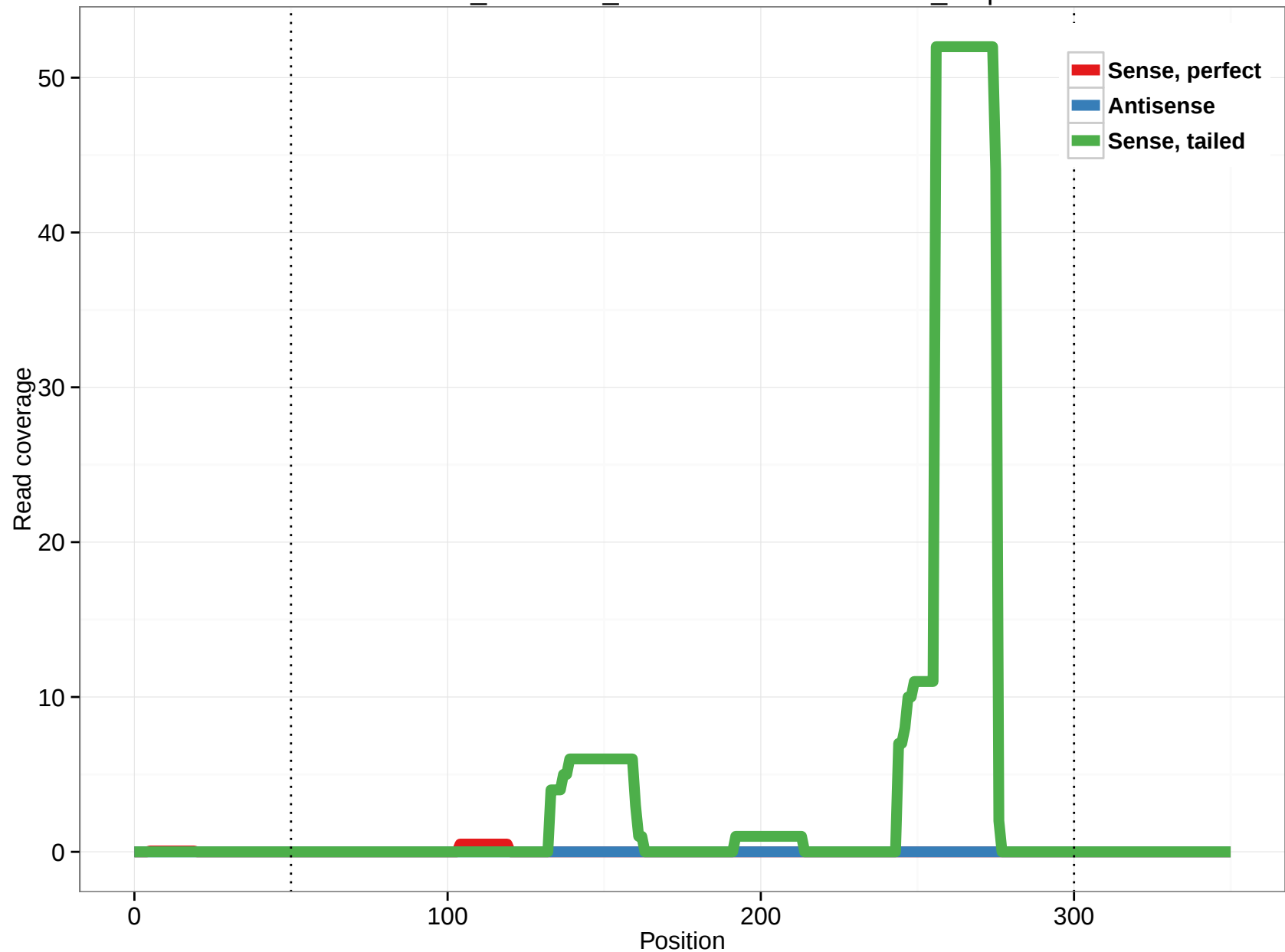
ornAna1_ensGene_ENSOANT00000002547_3.5p
