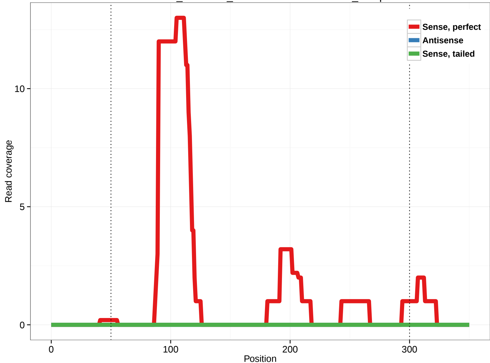
ornAna1_ensGene_ENSOANT00000002486_12.5p
