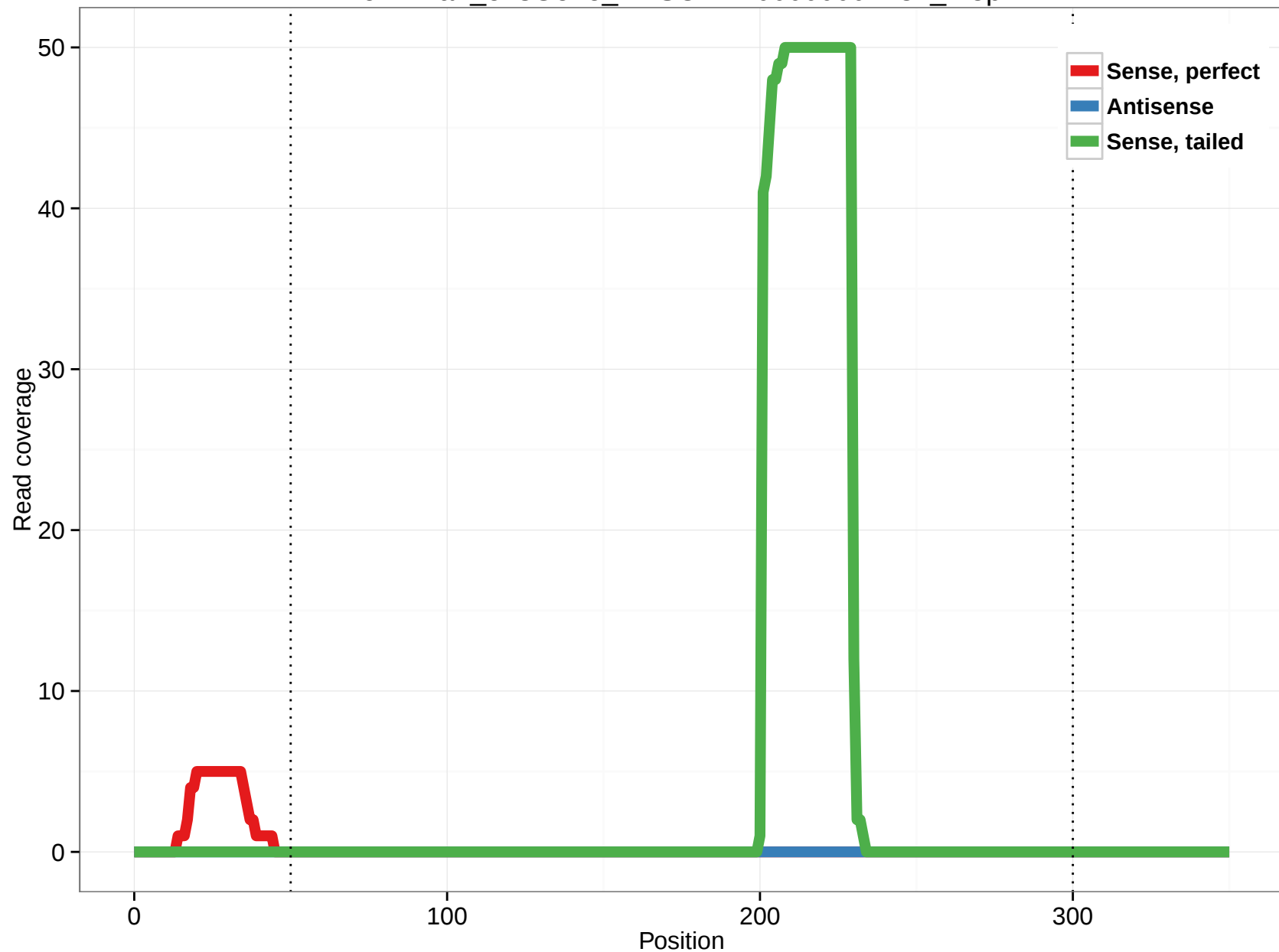
ornAna1_ensGene_ENSOANT00000002481_2.5p
