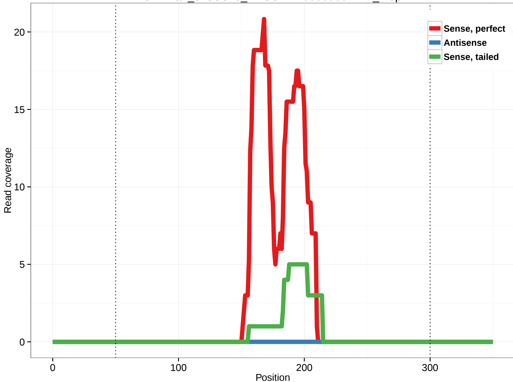
ornAna1_ensGene_ENSOANT00000002472_1.3p
