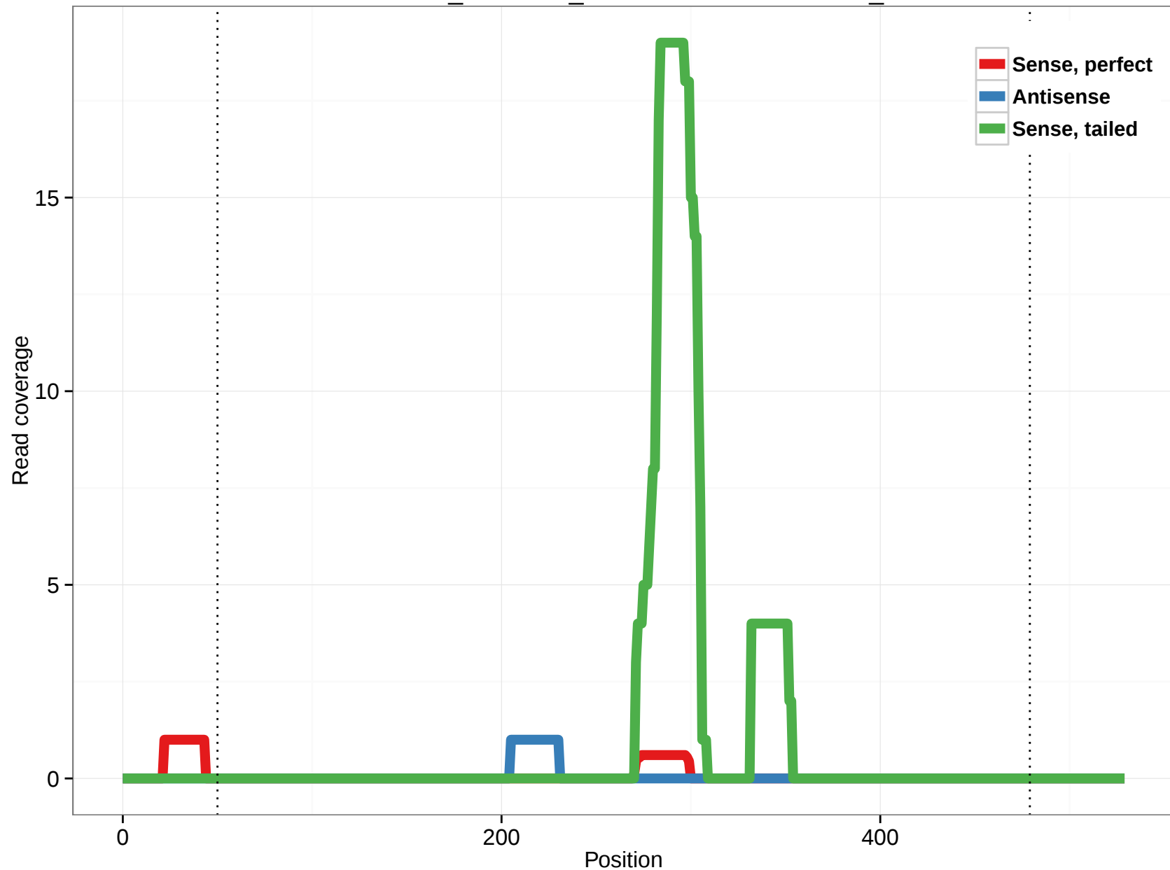
ornAna1_ensGene_ENSOANT00000002417_6
