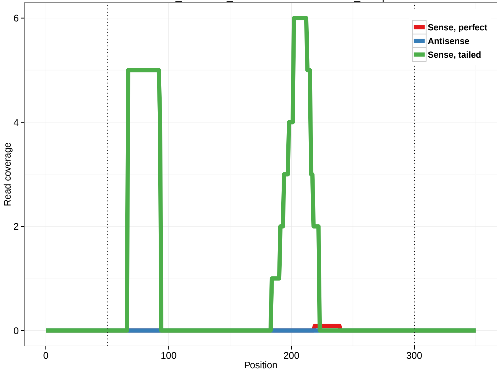
ornAna1_ensGene_ENSOANT00000002380_18.5p
