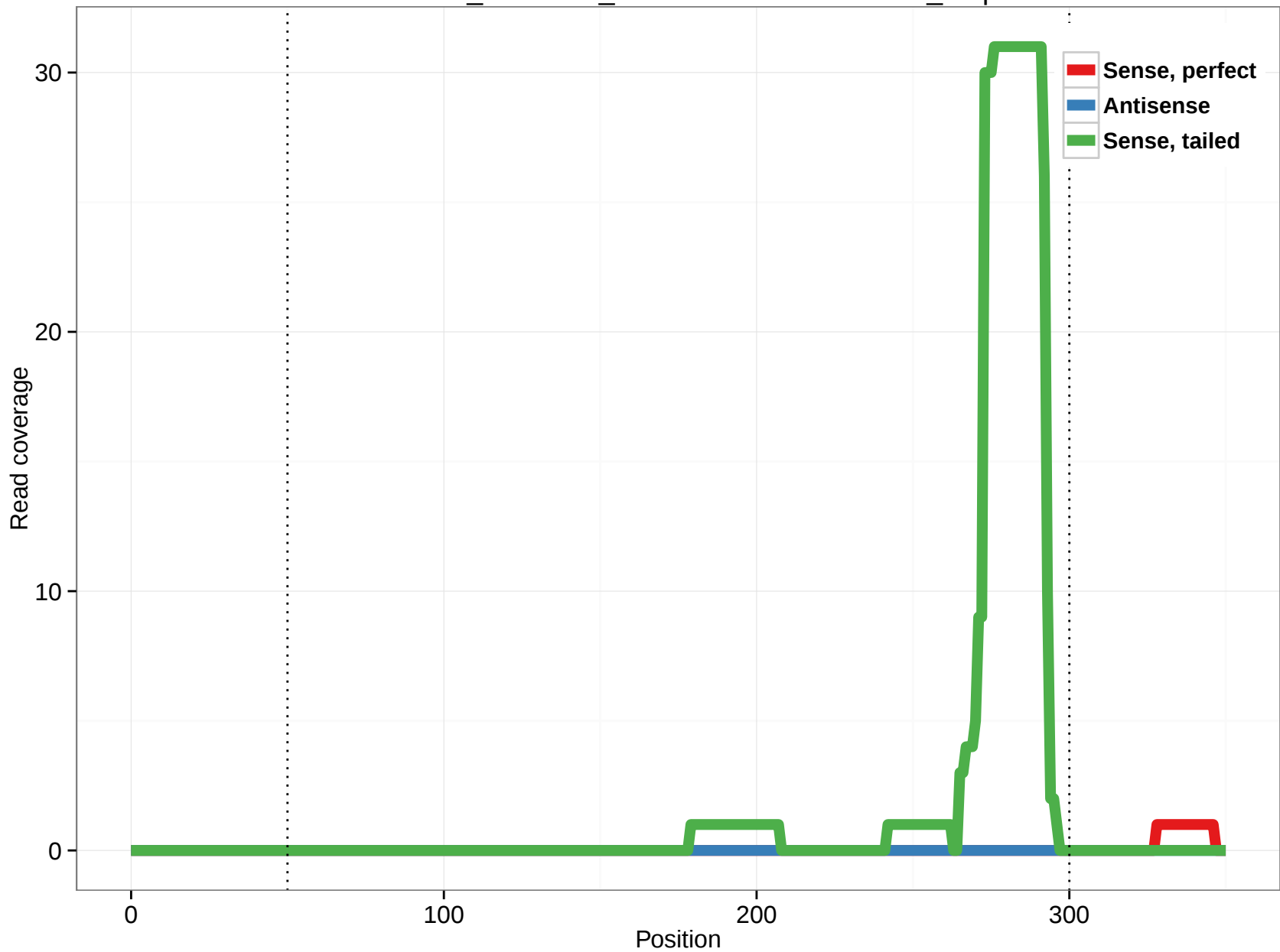
ornAna1_ensGene_ENSOANT00000002361_2.3p
