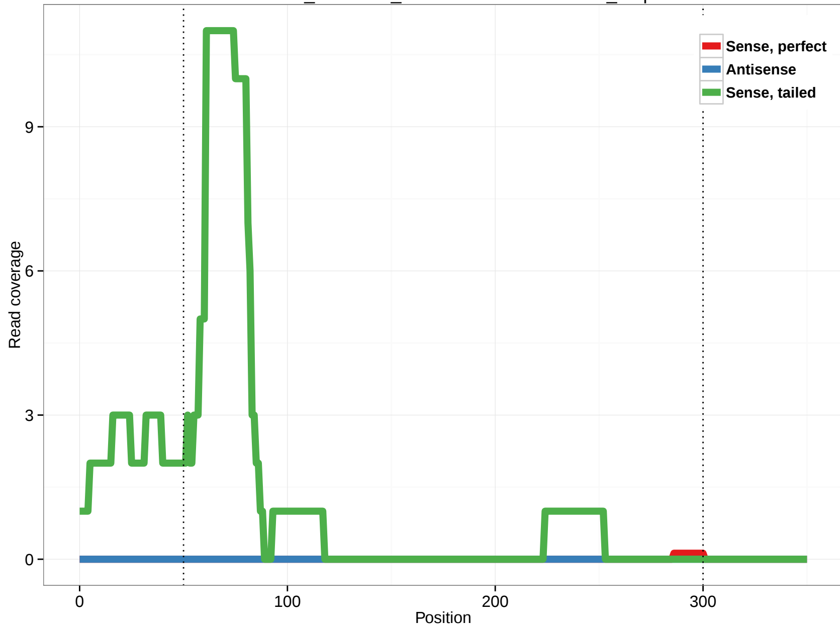
ornAna1_ensGene_ENSOANT00000002341_1.3p
