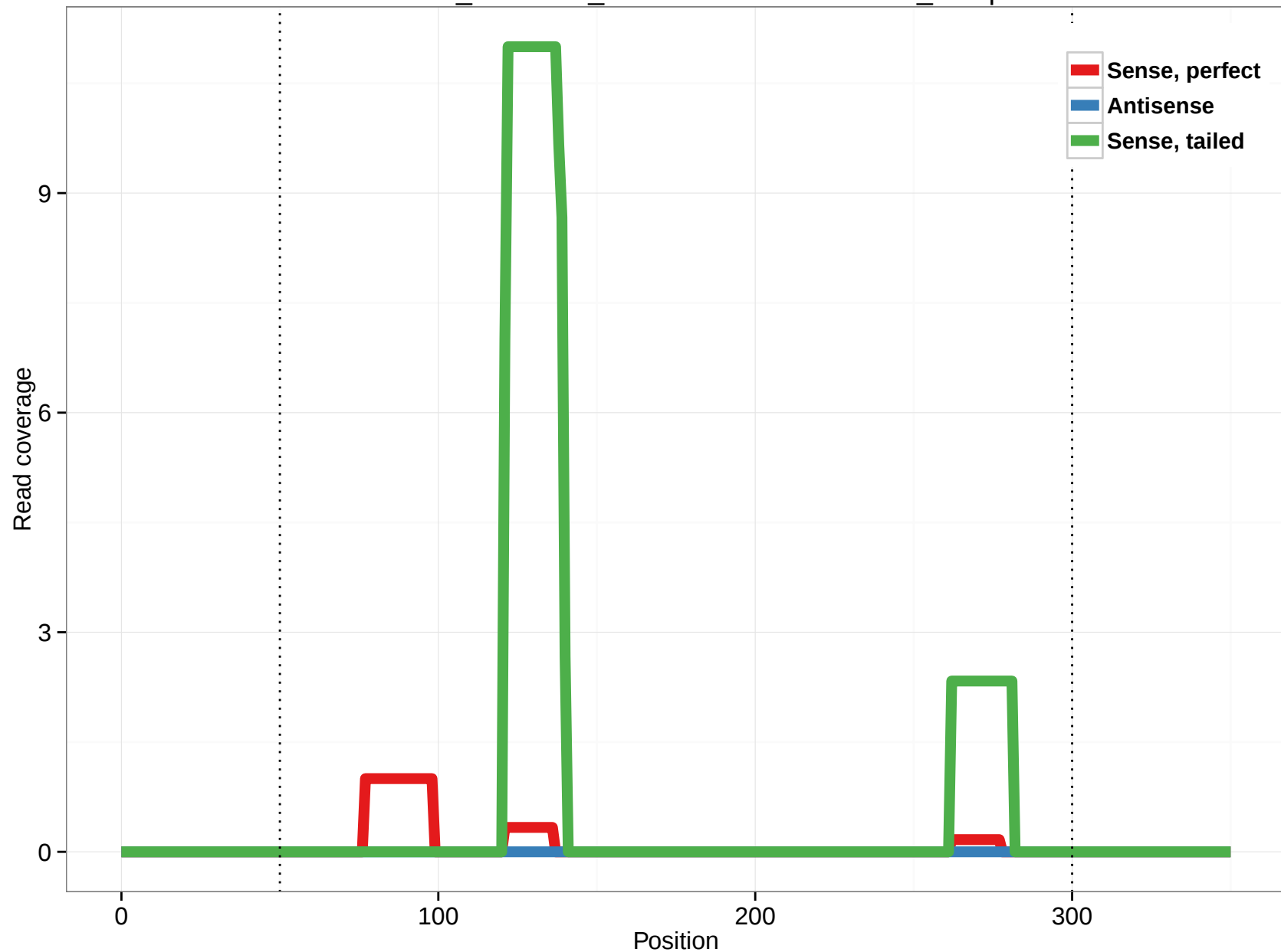
ornAna1_ensGene_ENSOANT00000002293_11.3p
