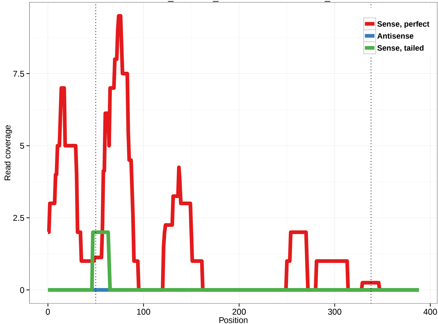
ornAna1_ensGene_ENSOANT00000002270_6
