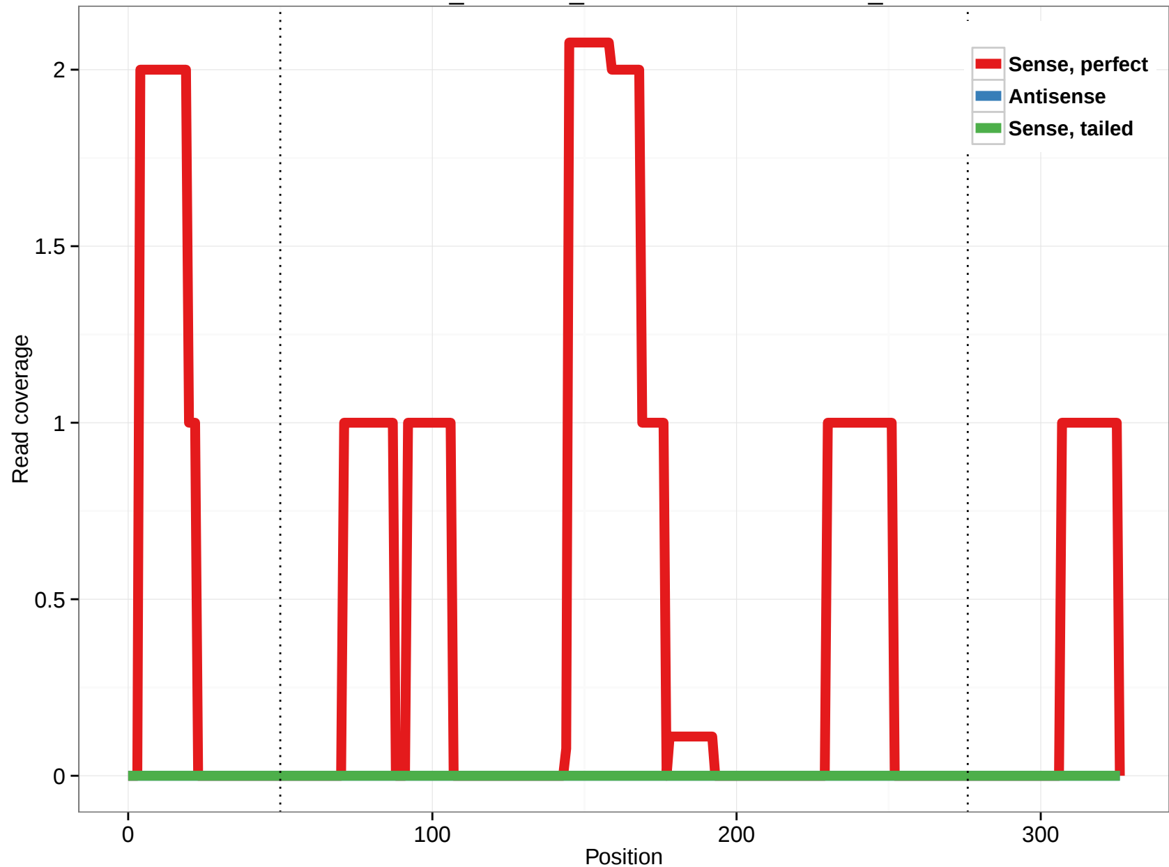
ornAna1_ensGene_ENSOANT00000002203_5
