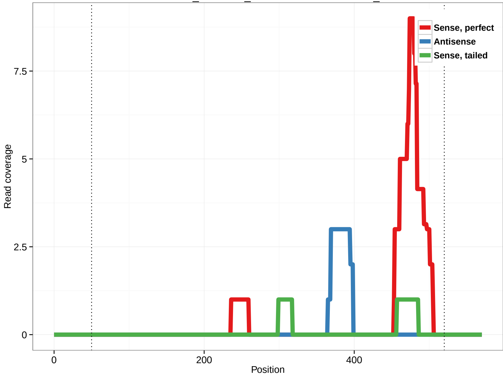
ornAna1_ensGene_ENSOANT00000002180_6
