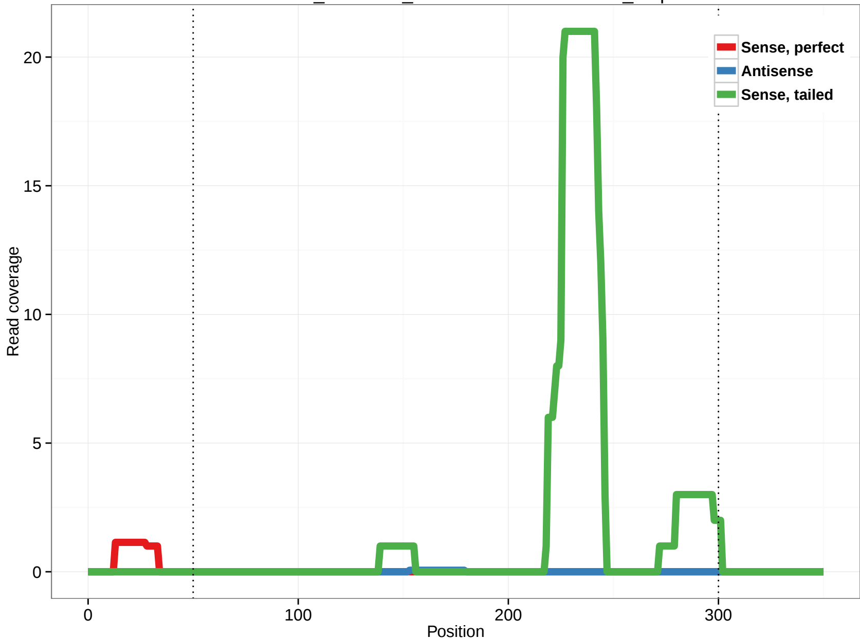
ornAna1_ensGene_ENSOANT00000002115_1.5p
