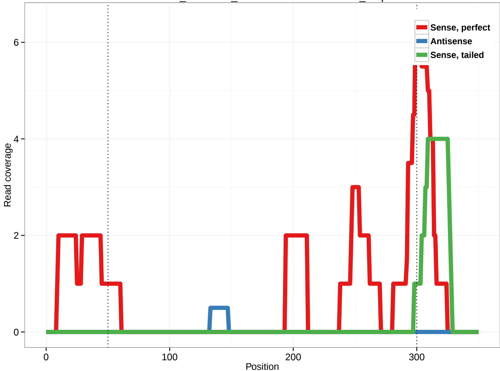
ornAna1_ensGene_ENSOANT00000002110_7.5p
