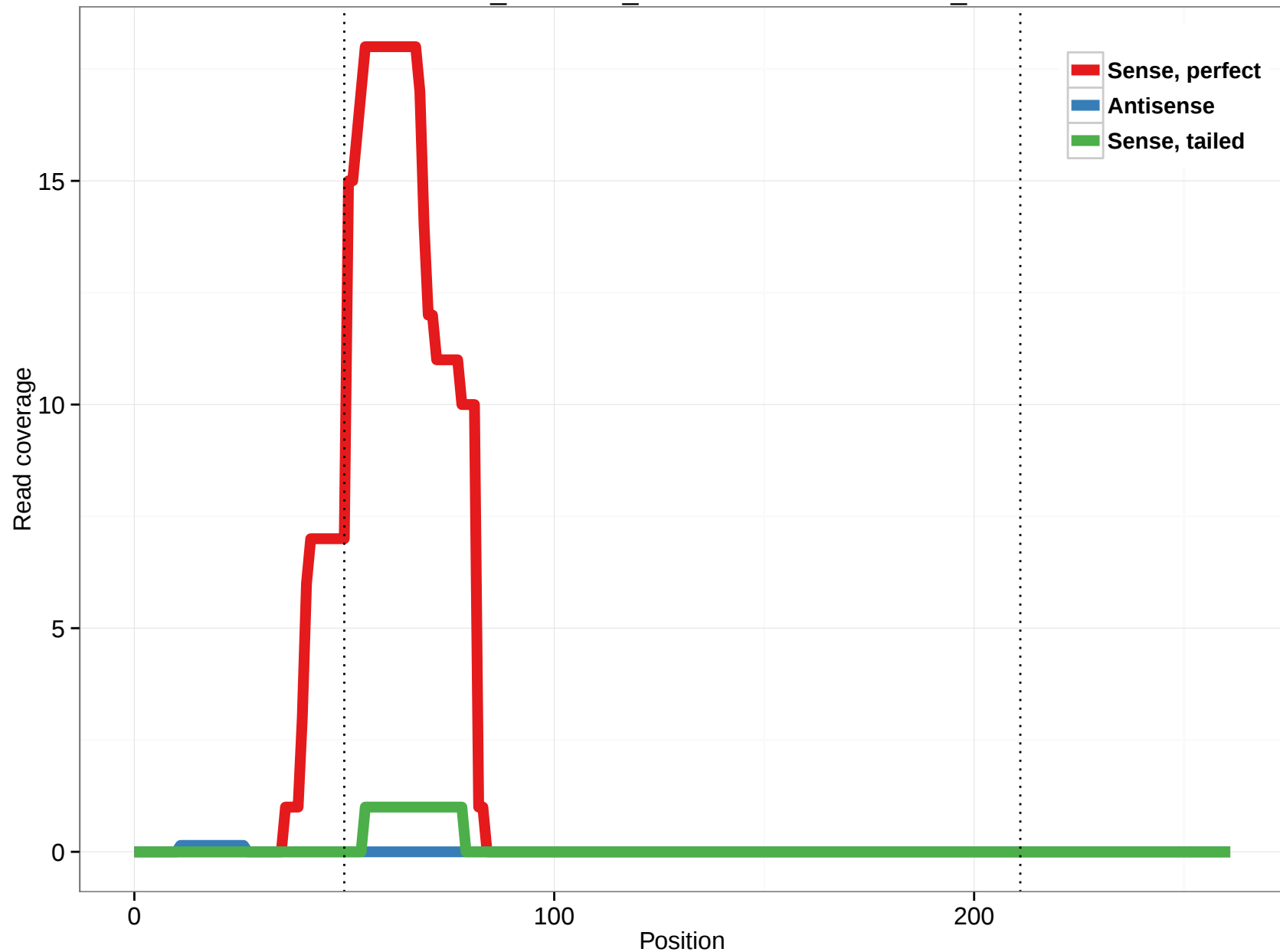
ornAna1_ensGene_ENSOANT00000002105_2
