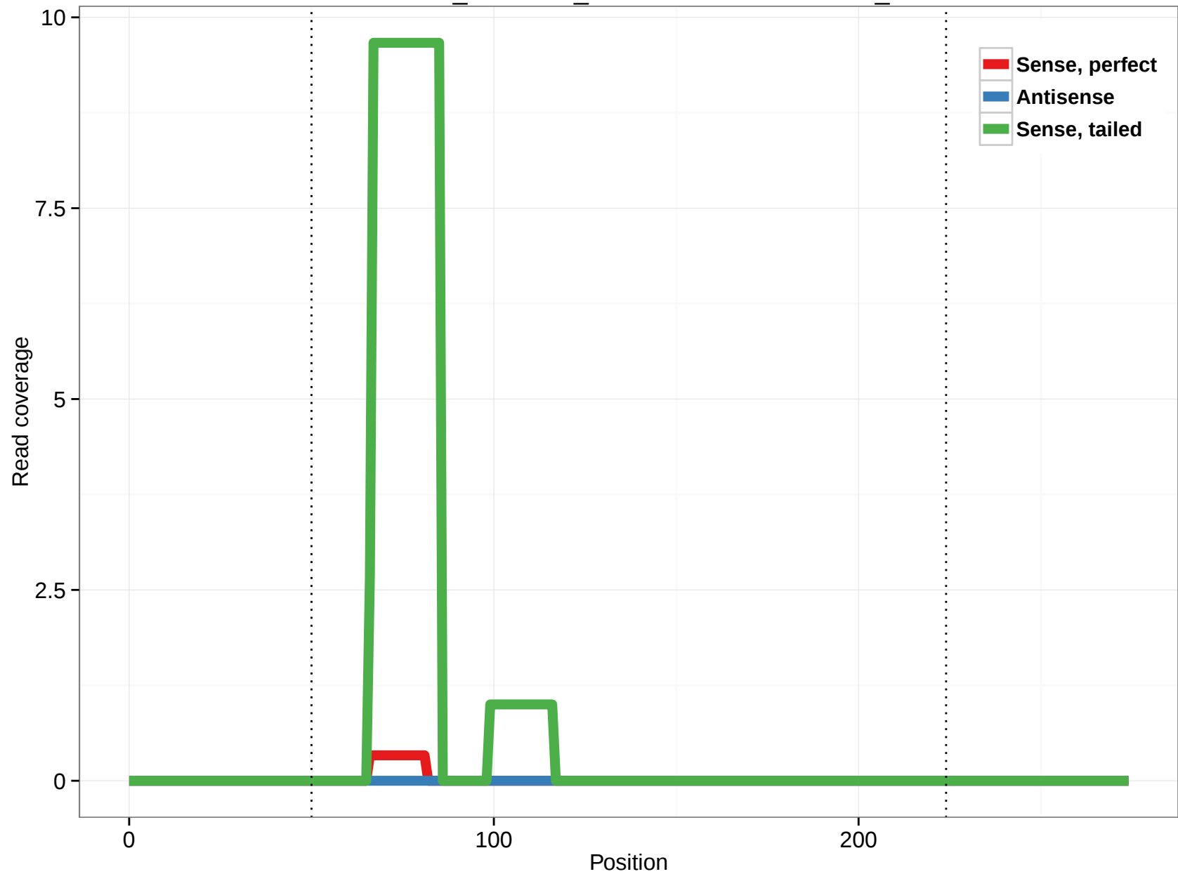
ornAna1_ensGene_ENSOANT00000002043_0
