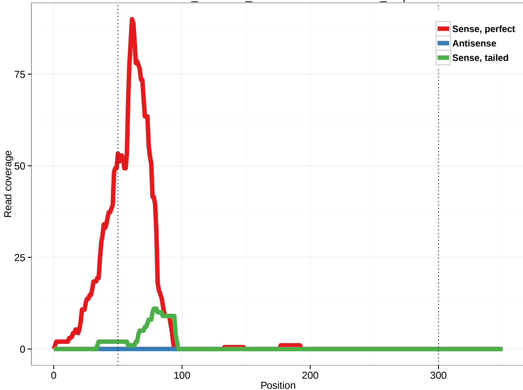
ornAna1_ensGene_ENSOANT00000002000_3.5p
