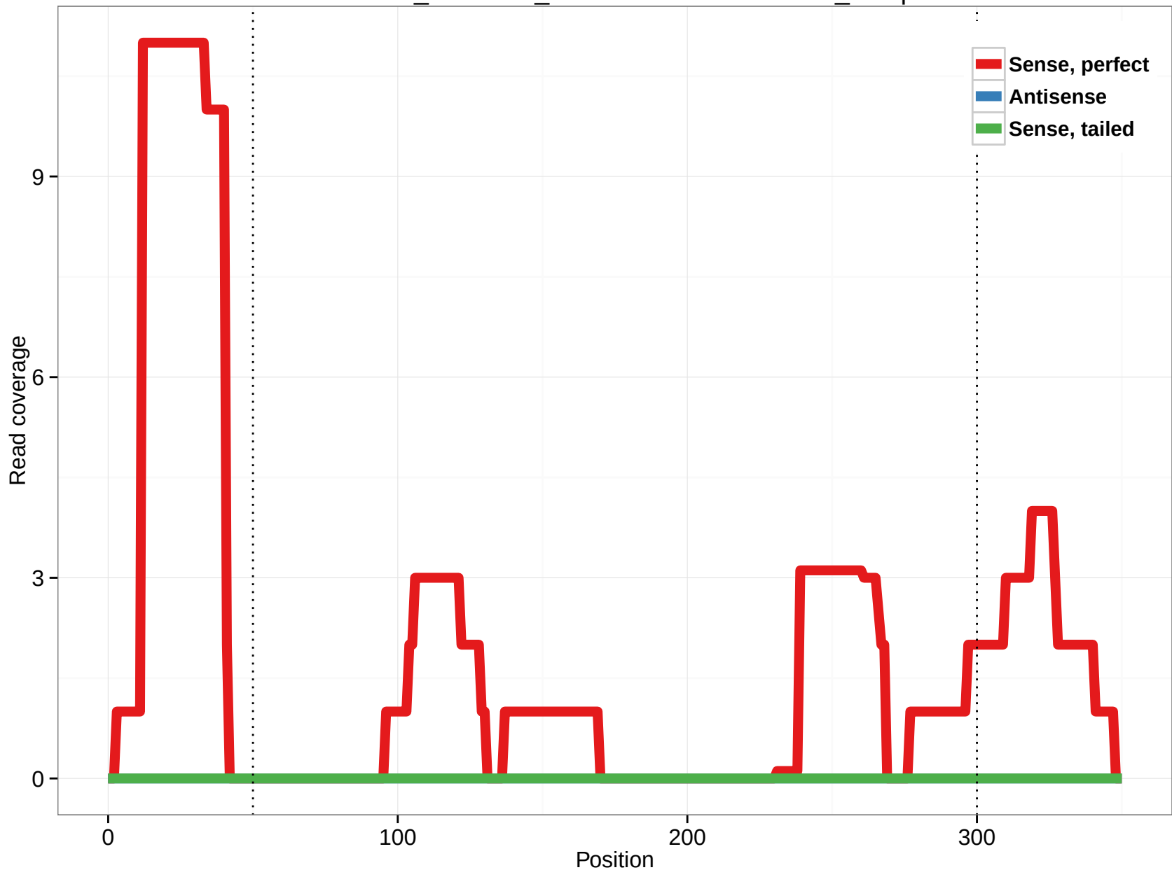
ornAna1_ensGene_ENSOANT00000001986_19.3p
