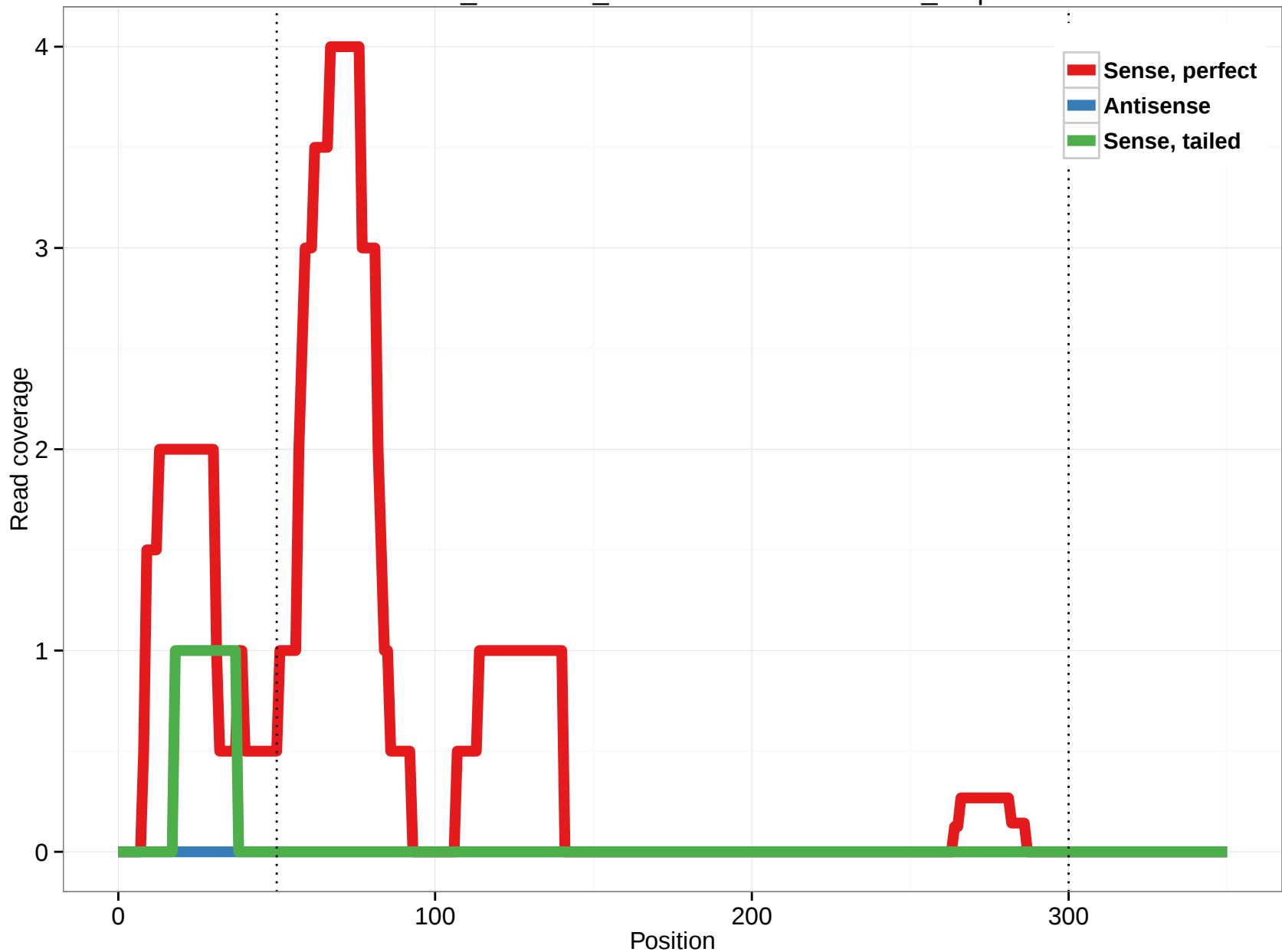
ornAna1_ensGene_ENSOANT00000001986_0.5p
