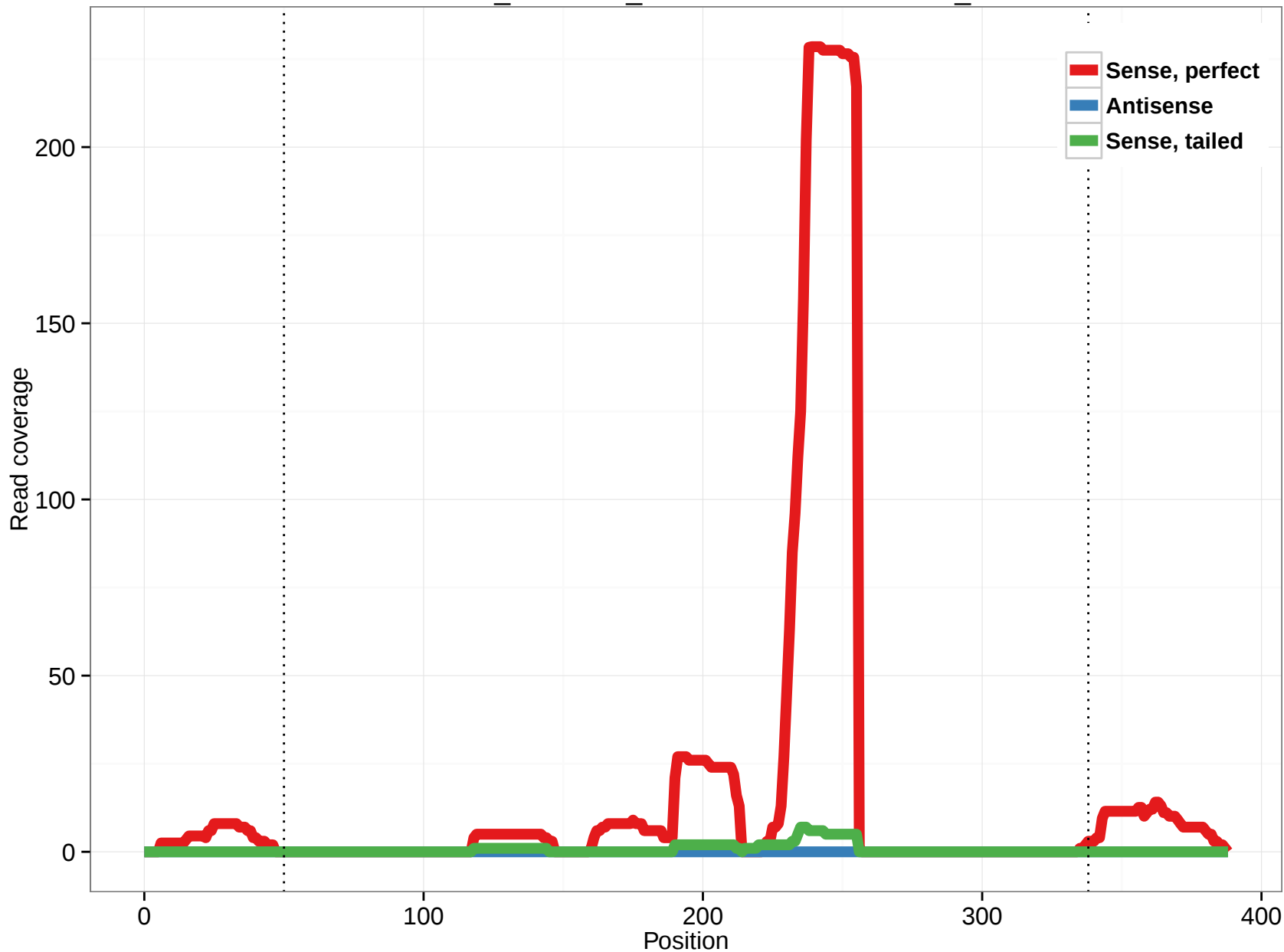
ornAna1_ensGene_ENSOANT00000001962_1
