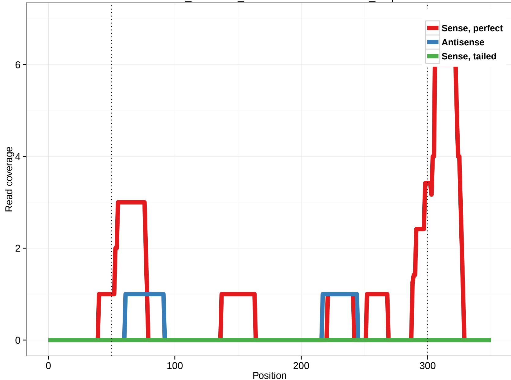
ornAna1_ensGene_ENSOANT00000001932_2.3p
