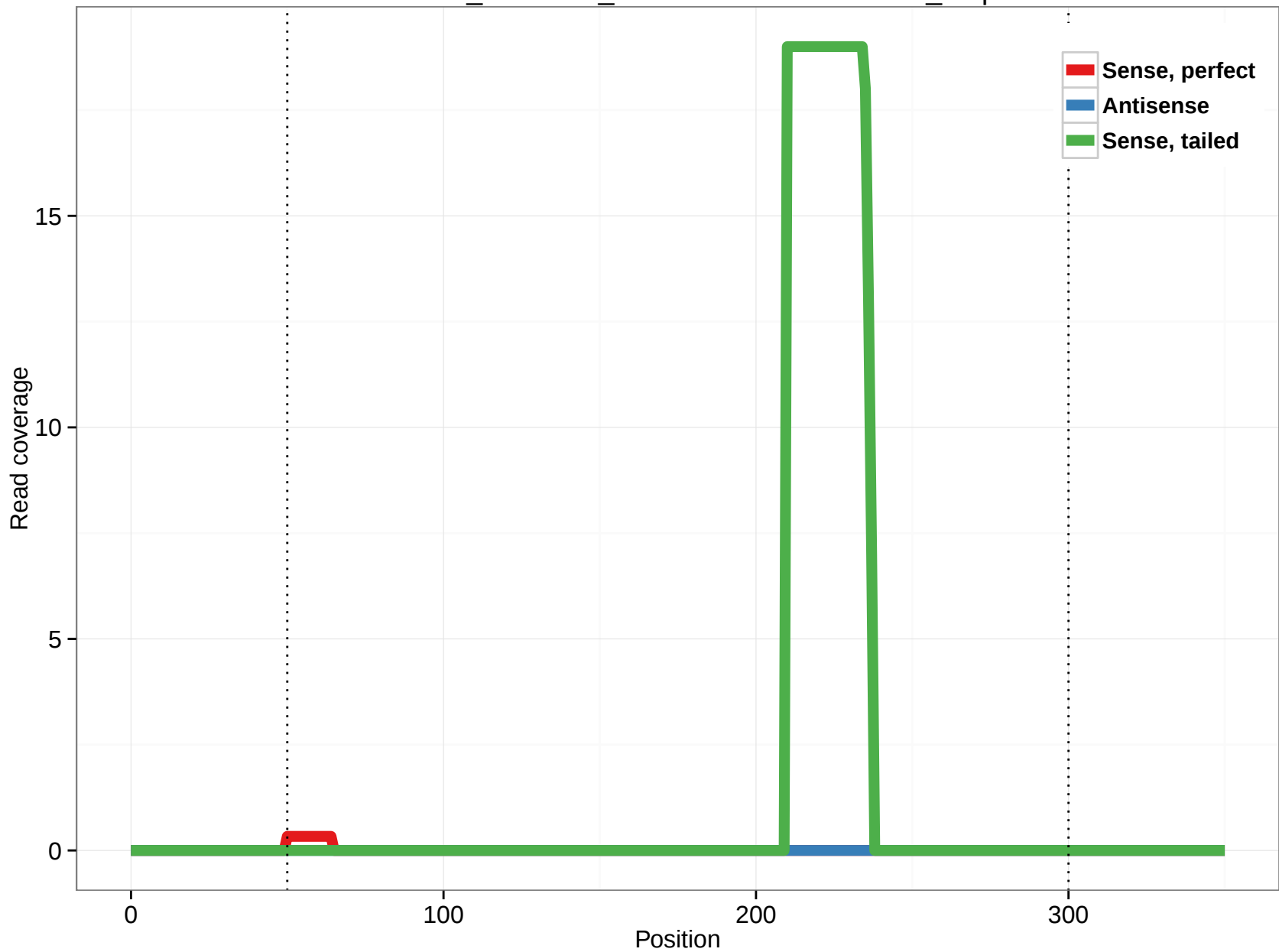
ornAna1_ensGene_ENSOANT00000001875_0.5p
