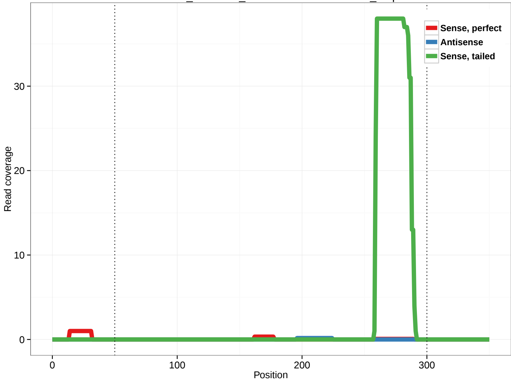
ornAna1_ensGene_ENSOANT00000001871_9.5p
