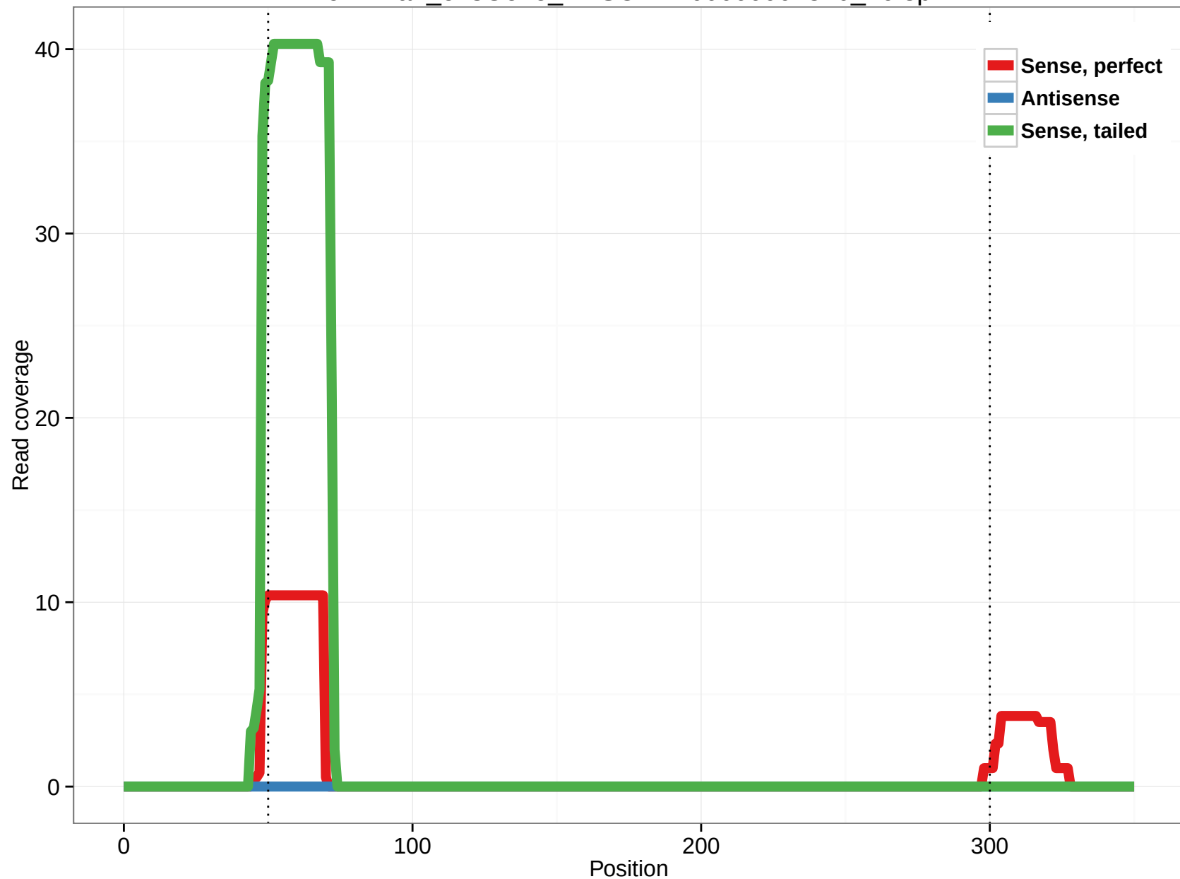
ornAna1_ensGene_ENSOANT00000001870_26.3p
