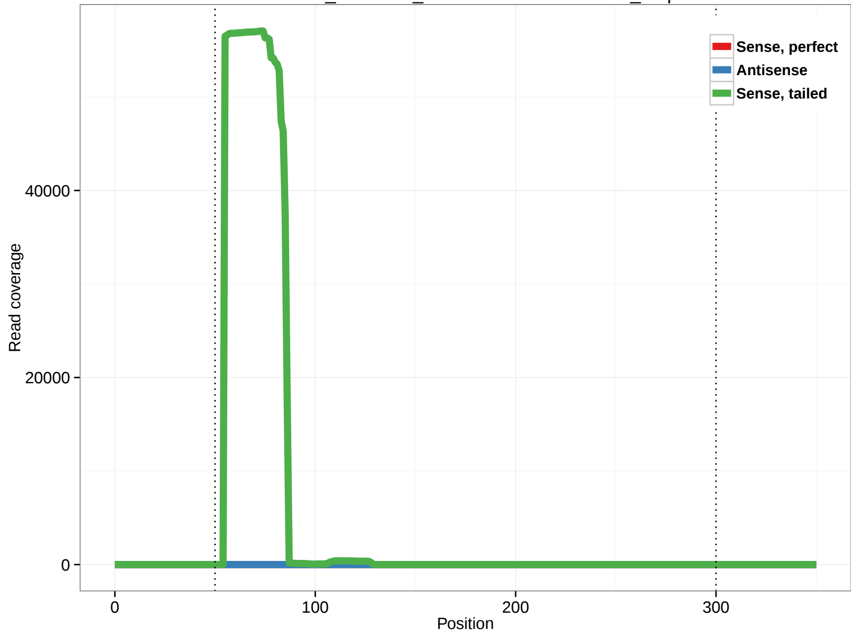
ornAna1_ensGene_ENSOANT00000001853_4.5p
