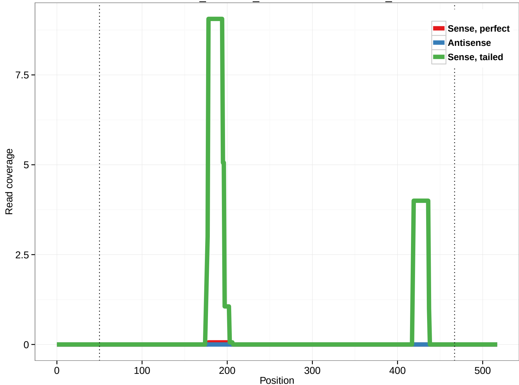
ornAna1_ensGene_ENSOANT00000001802_4
