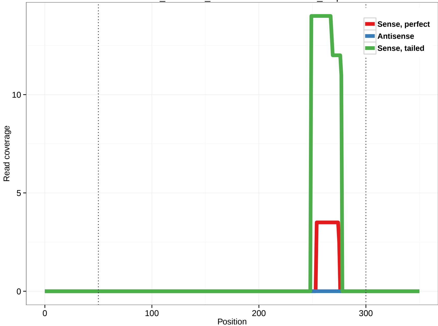
ornAna1_ensGene_ENSOANT00000001704_5.5p
