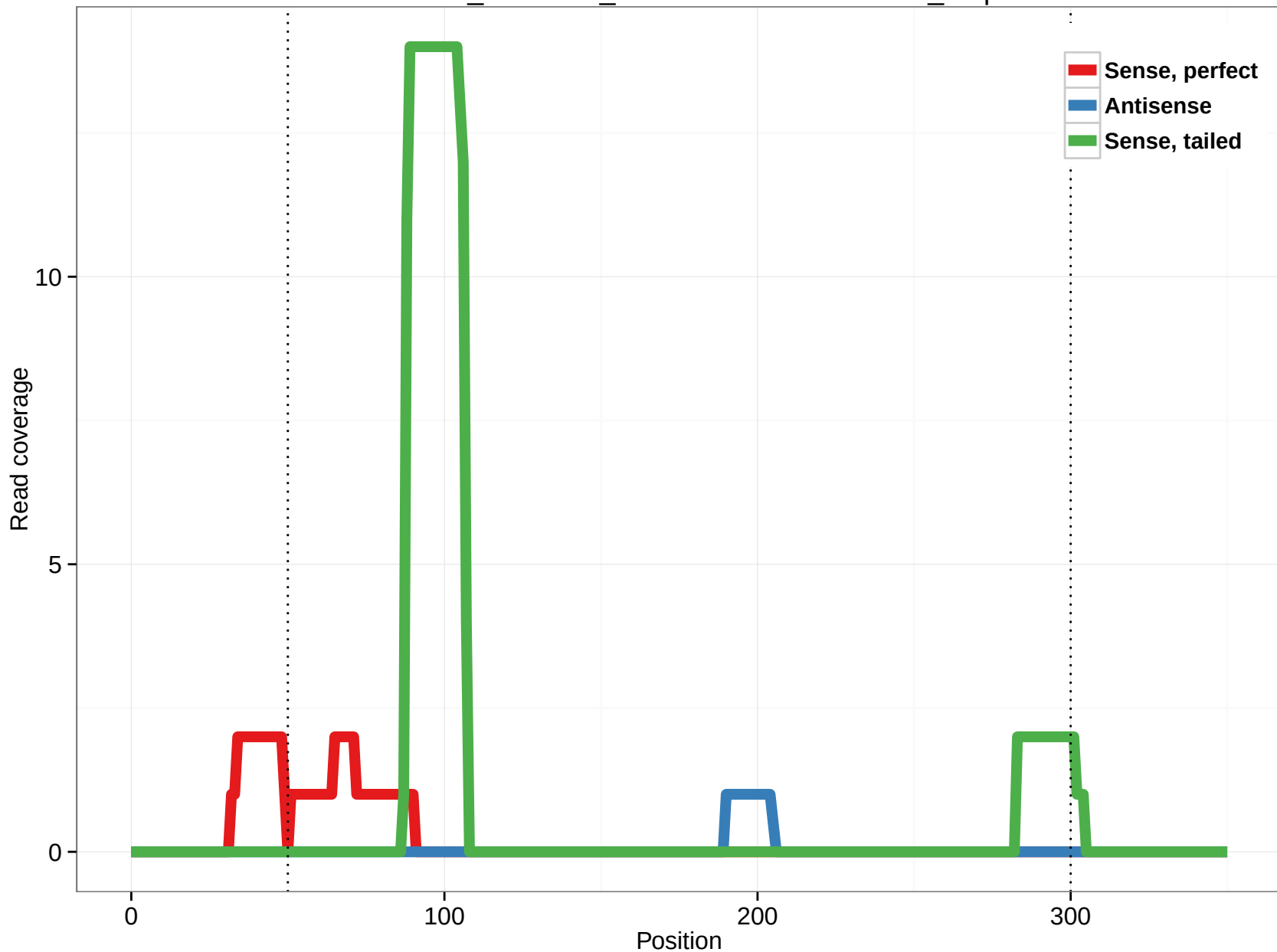
ornAna1_ensGene_ENSOANT00000001698_1.5p
