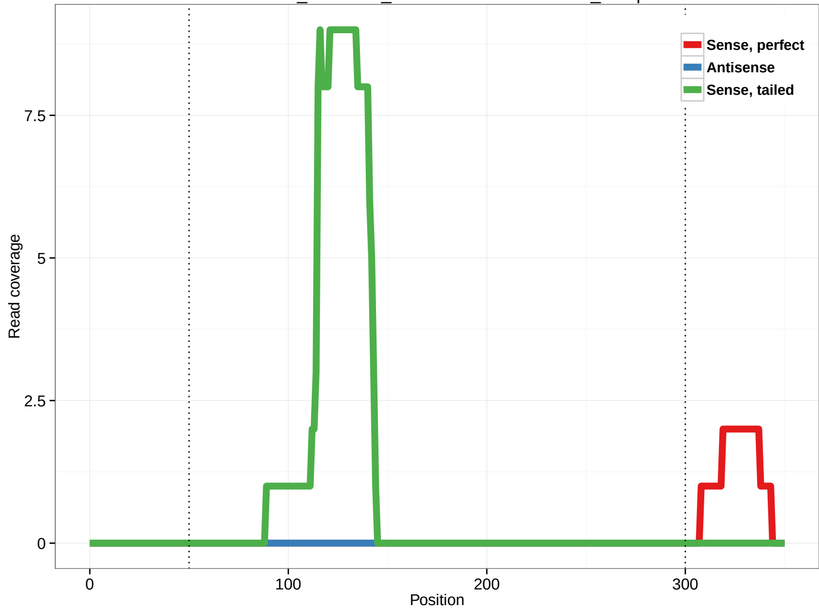
ornAna1_ensGene_ENSOANT00000001631_20.3p
