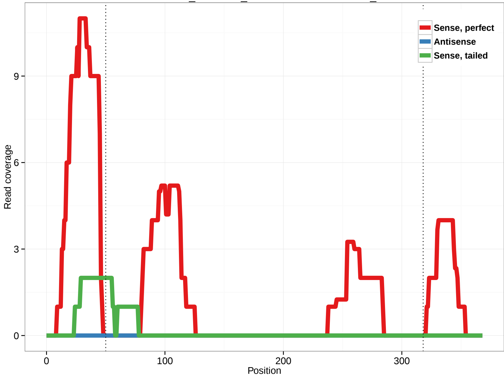
ornAna1_ensGene_ENSOANT00000001617_7
