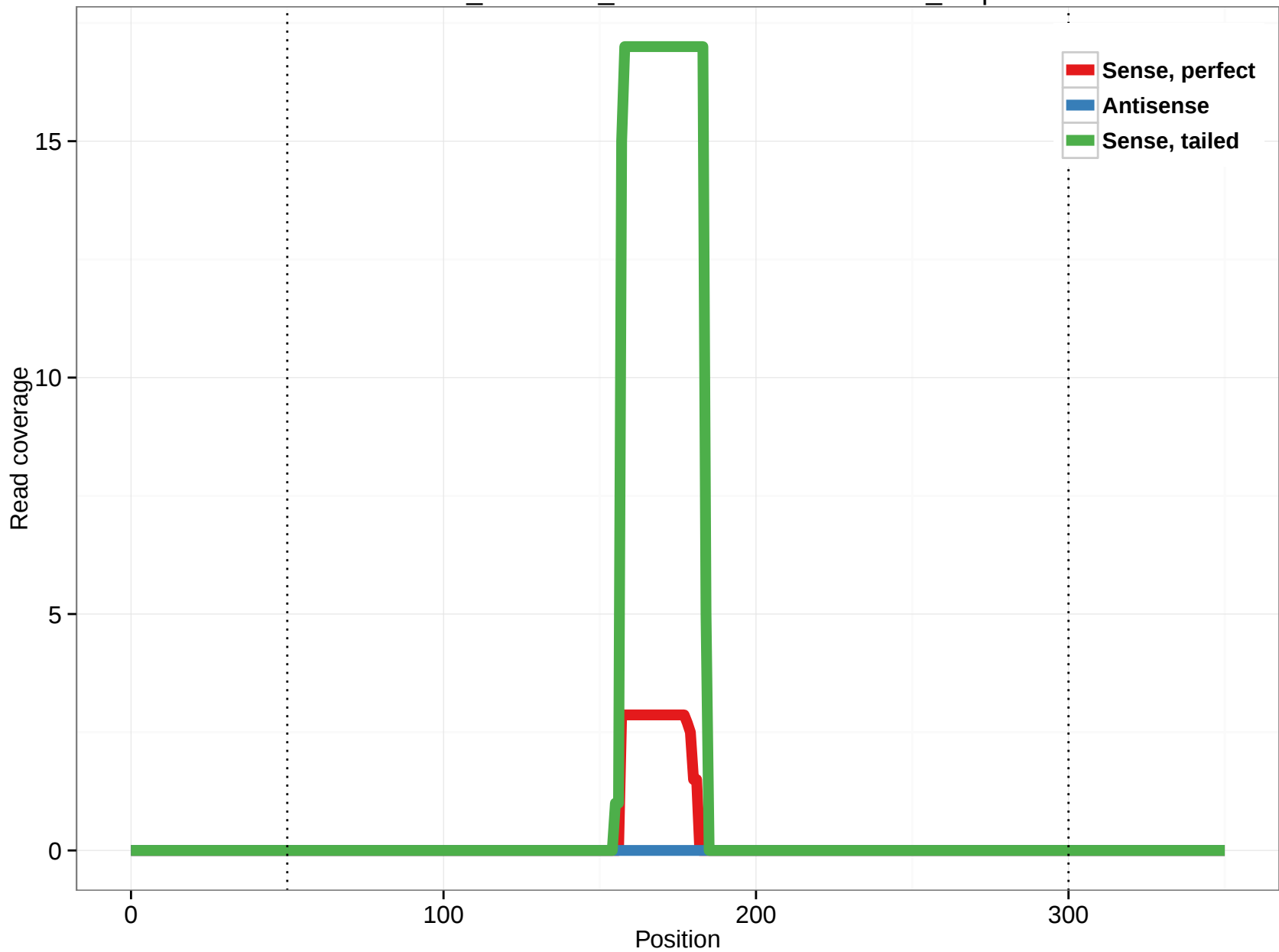
ornAna1_ensGene_ENSOANT00000001576_5.5p
