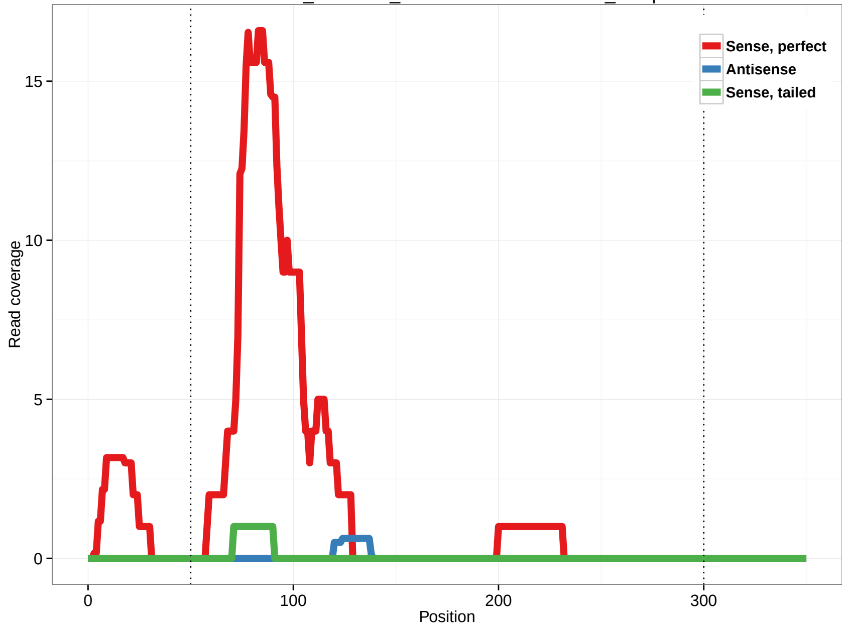
ornAna1_ensGene_ENSOANT00000001575_15.3p
