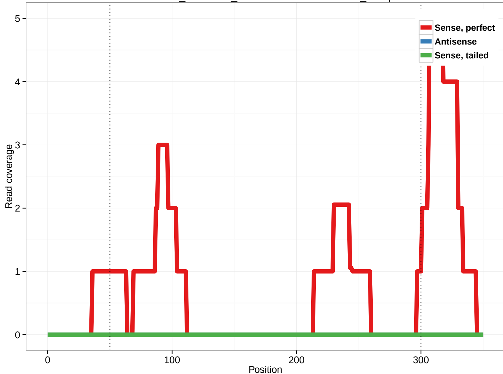
ornAna1_ensGene_ENSOANT00000001568_14.3p
