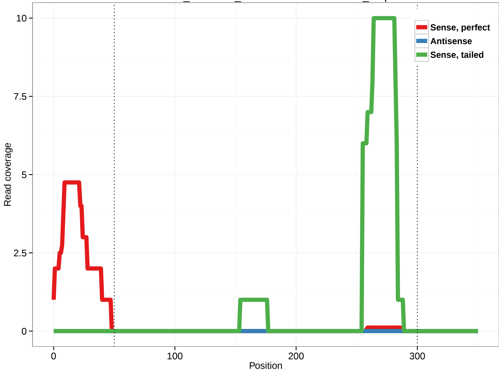
ornAna1_ensGene_ENSOANT00000001566_3.5p
