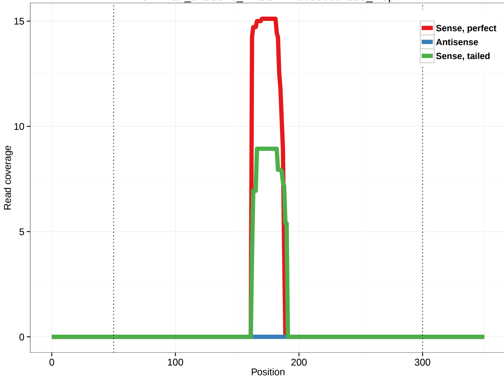
ornAna1_ensGene_ENSOANT00000001558_2.5p
