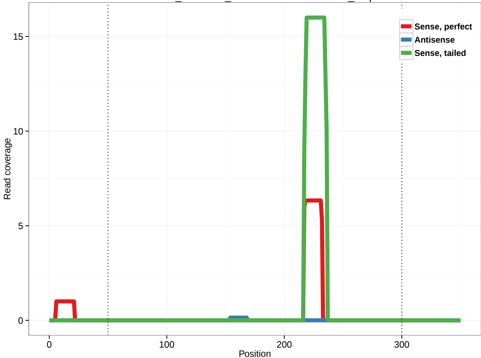
ornAna1_ensGene_ENSOANT00000001491_3.5p
