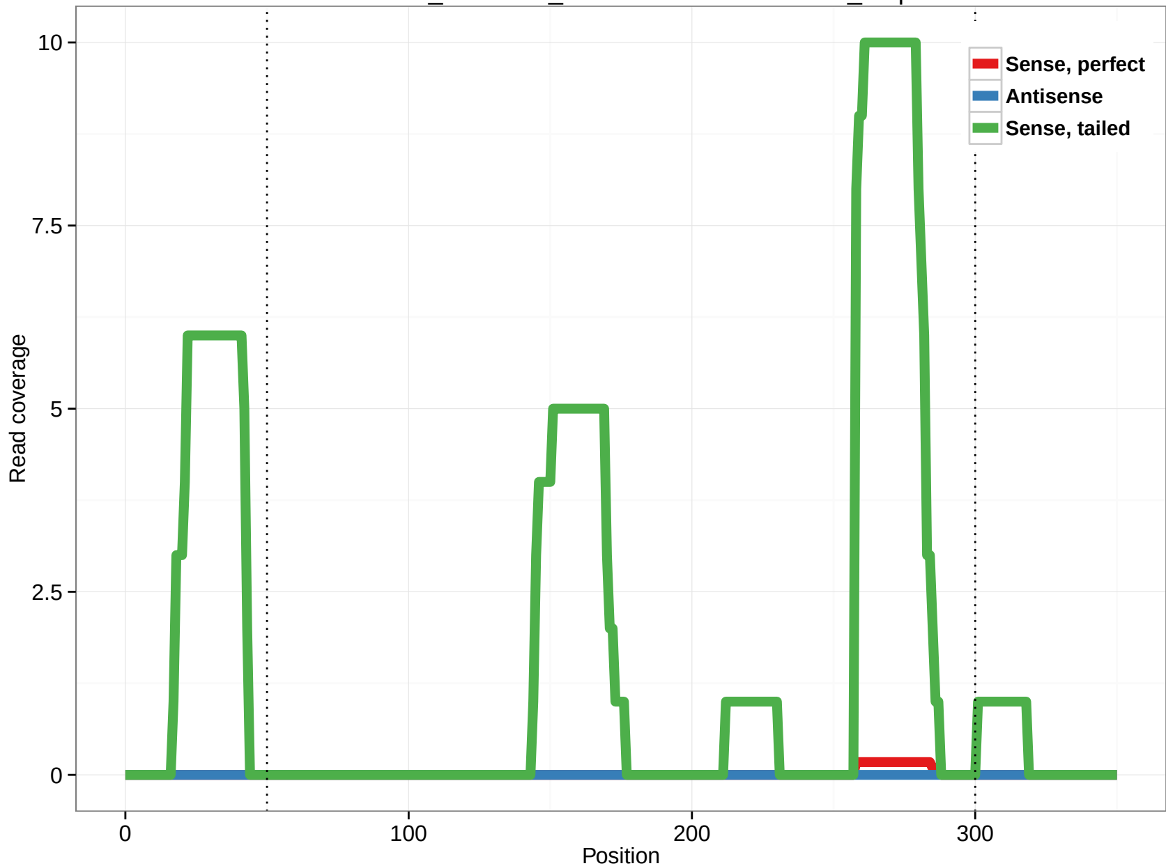
ornAna1_ensGene_ENSOANT00000001484_9.3p
