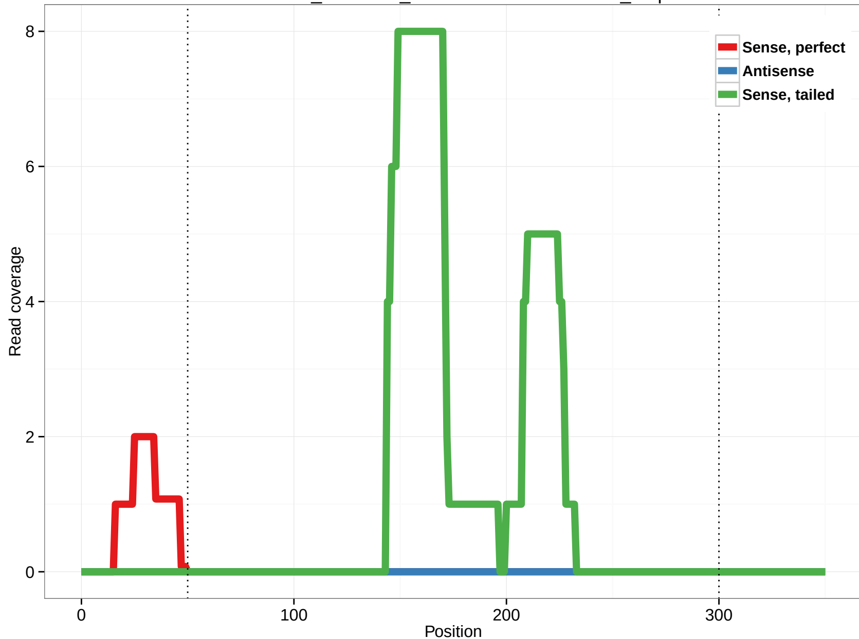
ornAna1_ensGene_ENSOANT00000001473_8.5p
