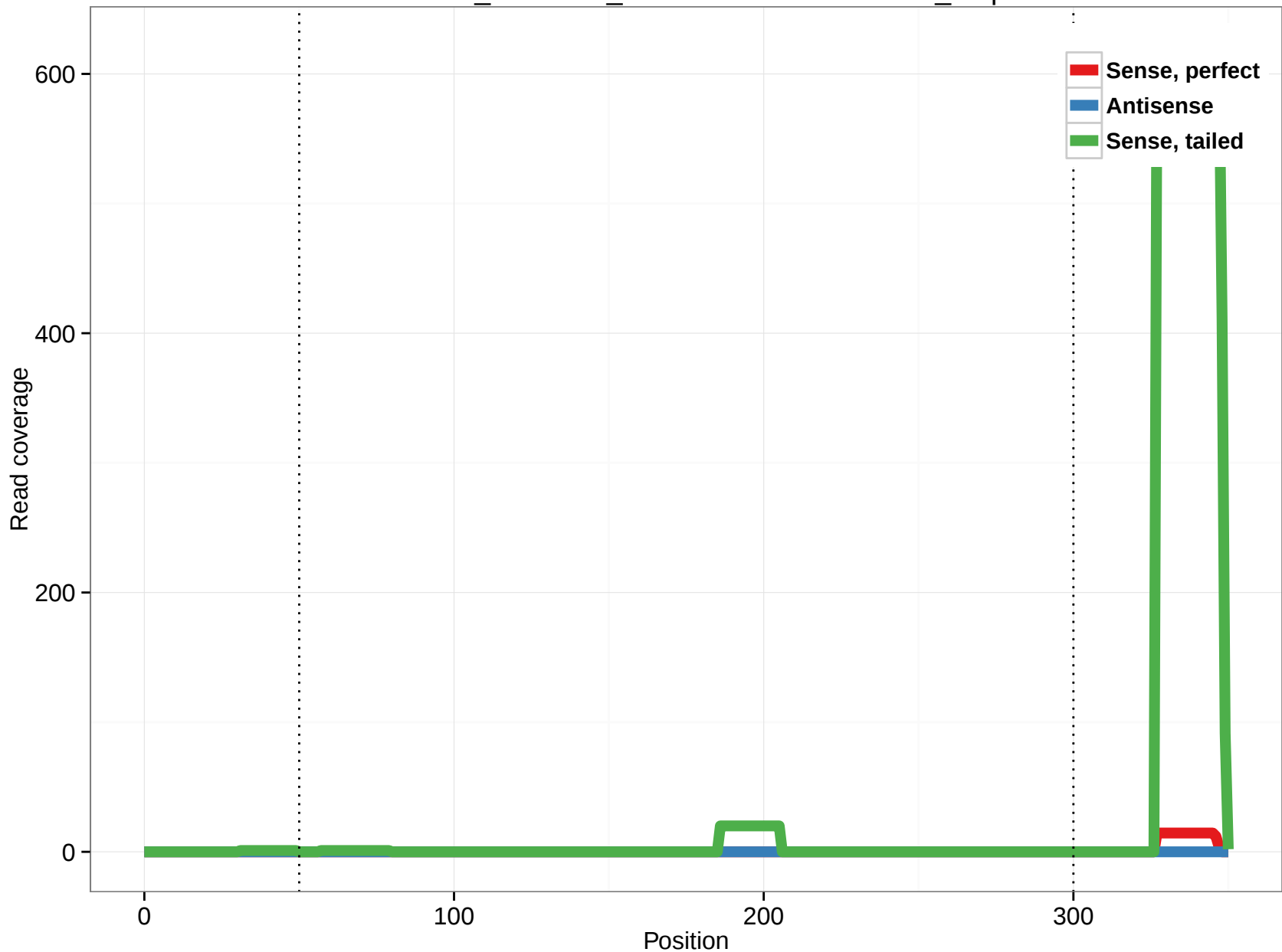
ornAna1_ensGene_ENSOANT00000001455_0.5p
