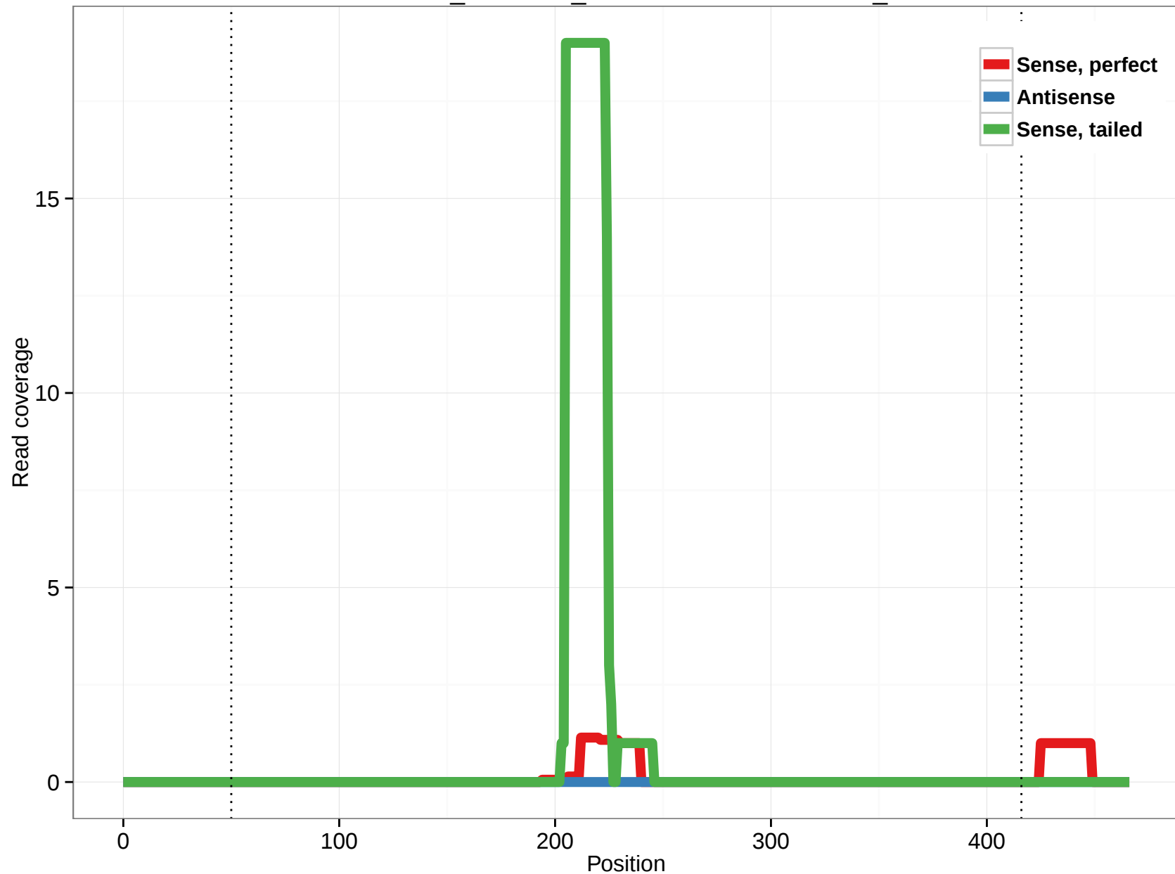
ornAna1_ensGene_ENSOANT00000001398_4
