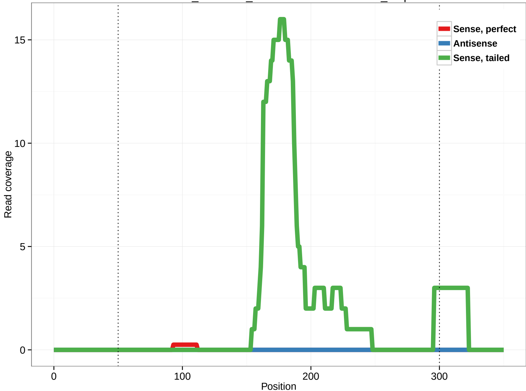
ornAna1_ensGene_ENSOANT00000001389_4.5p
