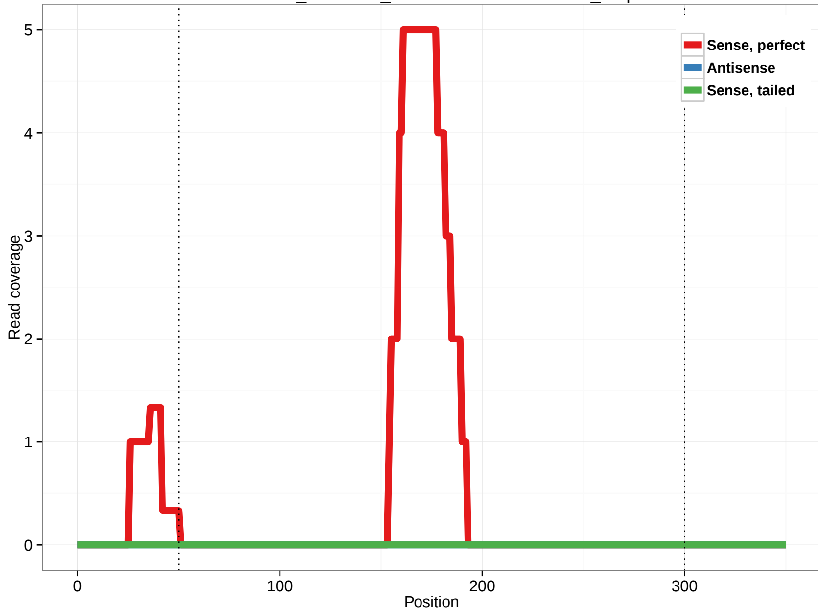
ornAna1_ensGene_ENSOANT00000001279_3.5p
