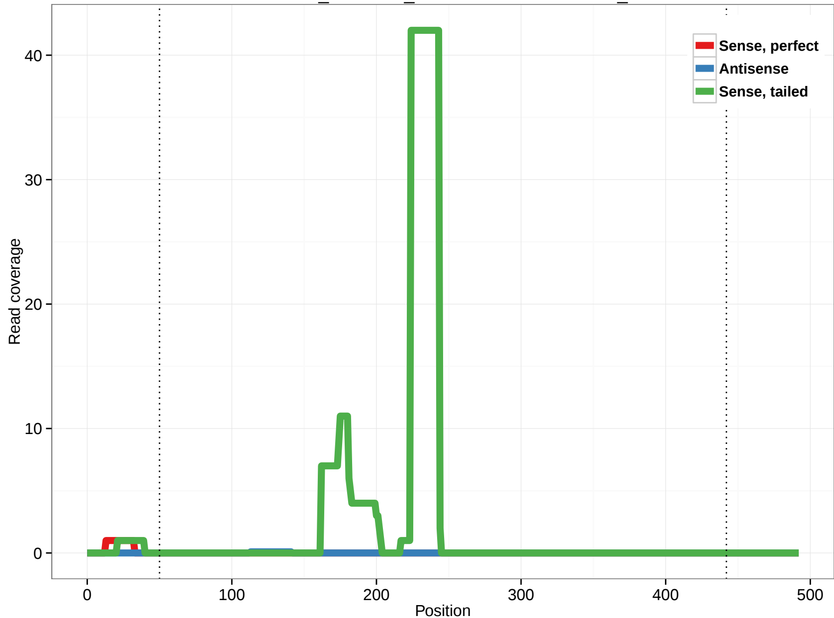
ornAna1_ensGene_ENSOANT00000001159_2
