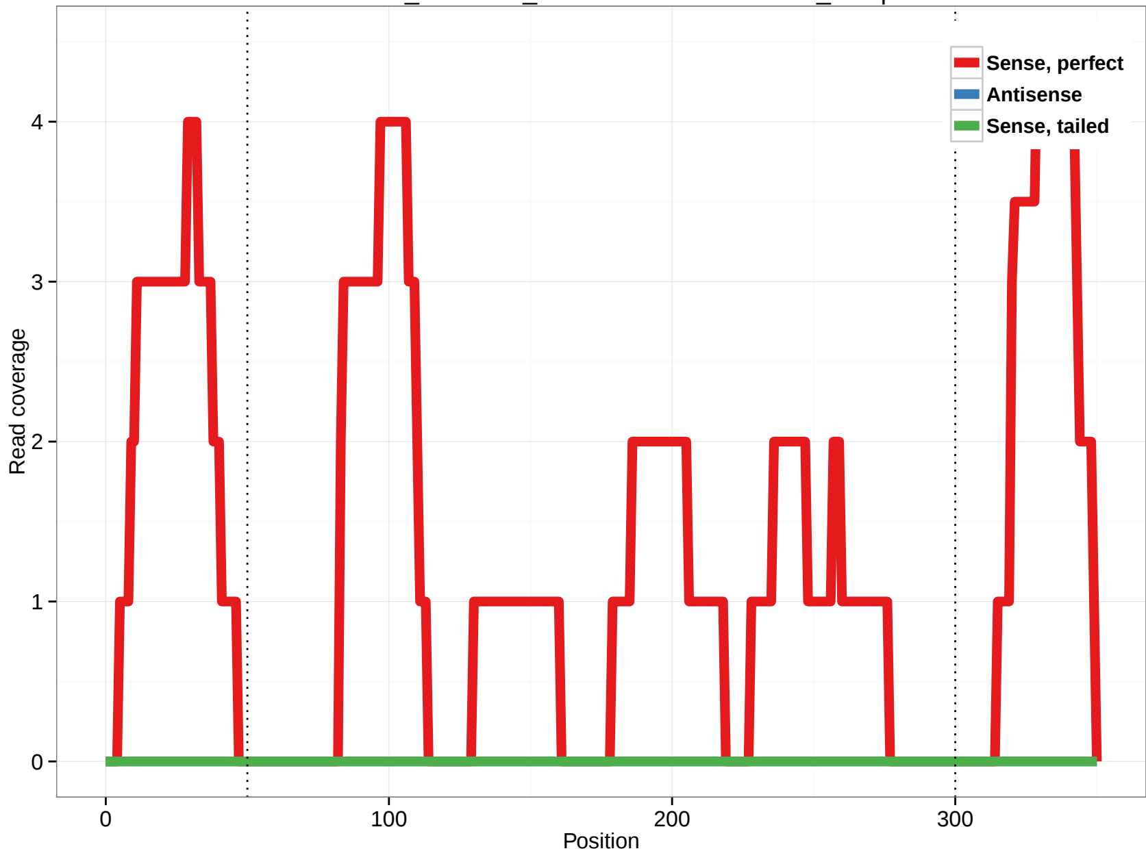
ornAna1_ensGene_ENSOANT00000001125_11.3p
